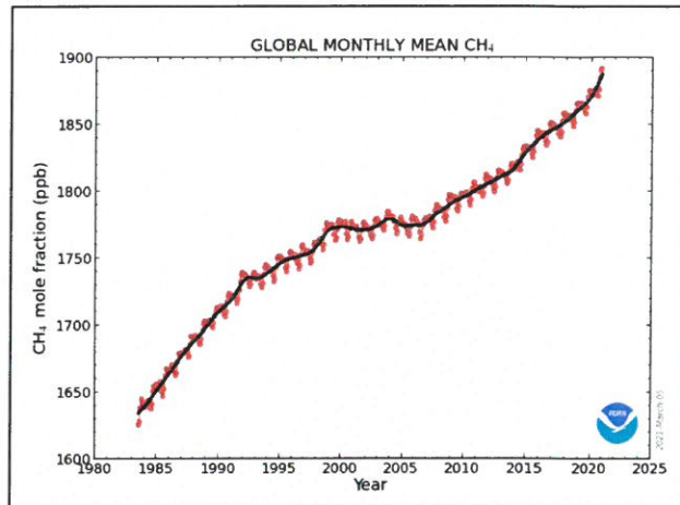
Figure 2. Mean monthly methane concentrations, 1983-2020
